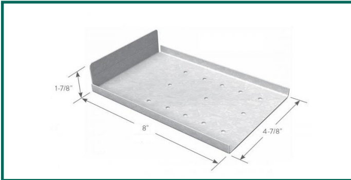
Extended Uni Clip™ (UXRC)
