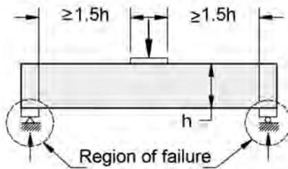
End One Flange Loading (EOF)
