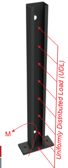
Uniformly distributed loads are based on framing members placed on each side of the Pony Wall
